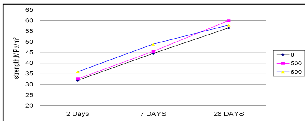
Figure. The relationship between the strength of cement and the time of rigidity at different doses of grinding aids. At (500) ml :
